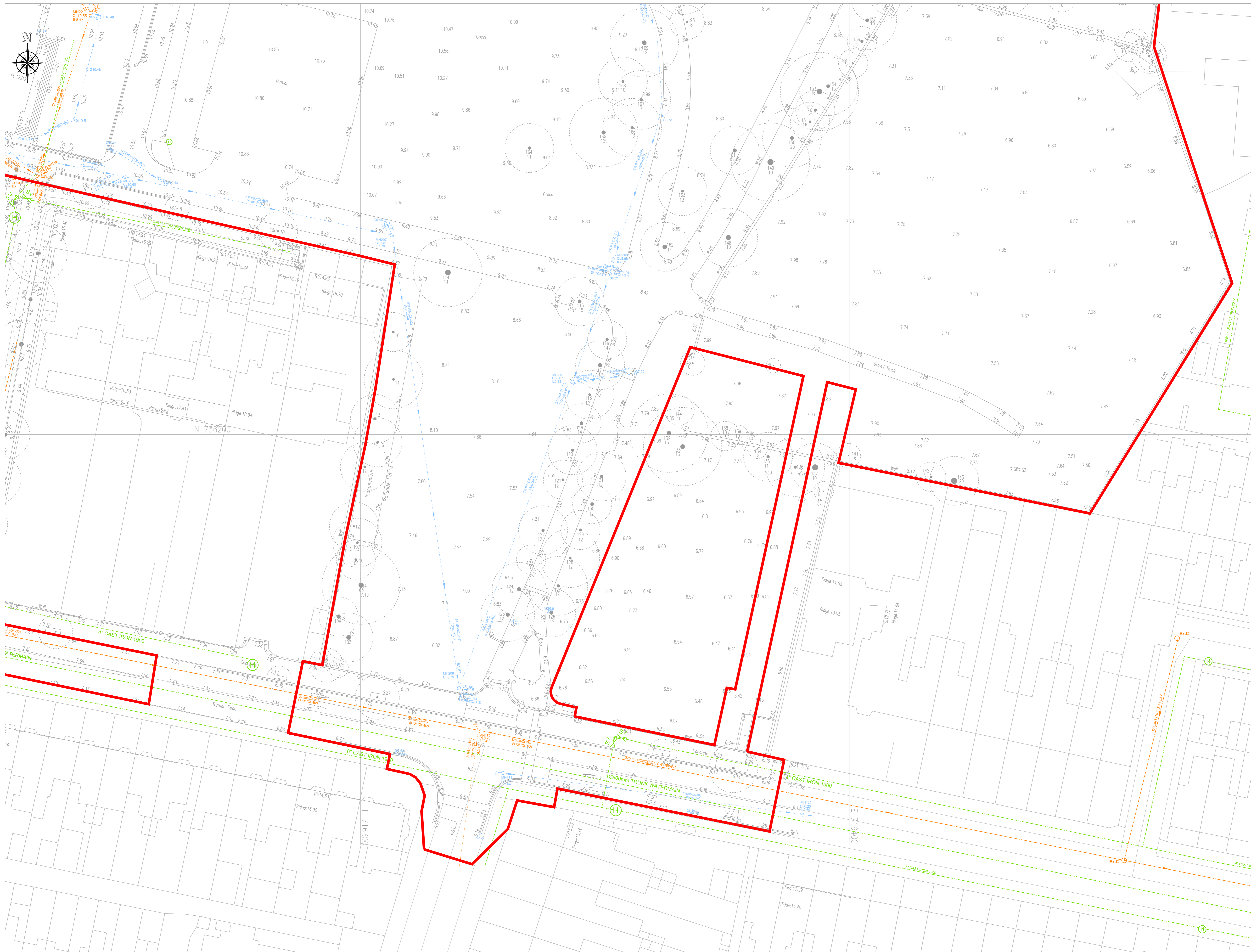
EXISTING BURIED DRAINAGE AND WATERMAIN PLAN LAYOUT - SHEET 4 OF 4 SCALE @ A0: 1:500 SCALE @ A2: 1:500
